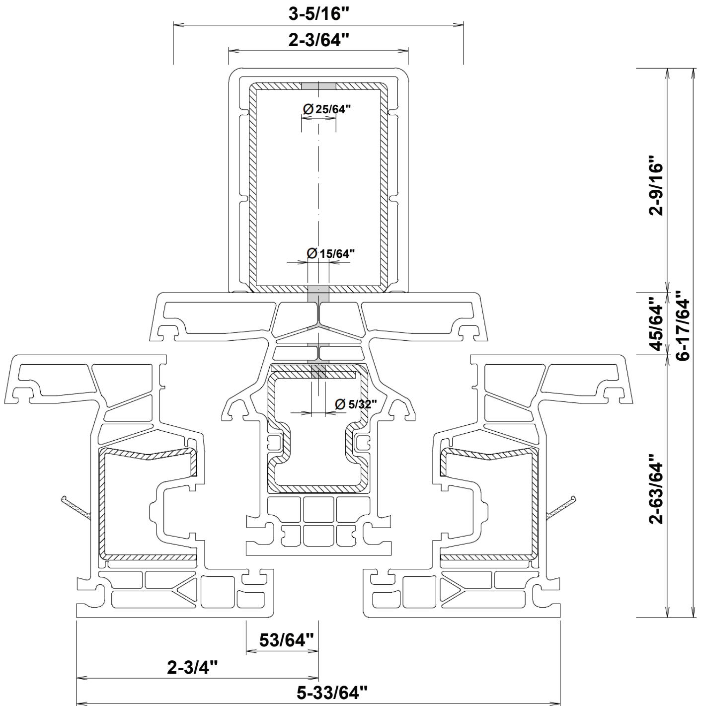
Cladding profile with external steel support (for transom sash profile)
