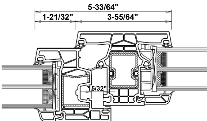
3-55/64" T-profile with side fixed - Premium KN76
