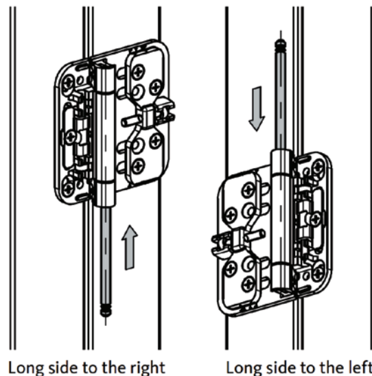
Installing the pin in the sash hinge
