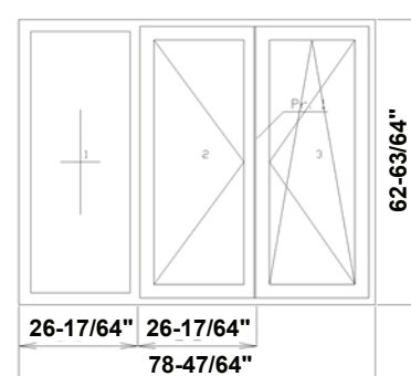
2 sash opening over 1 side fixed
