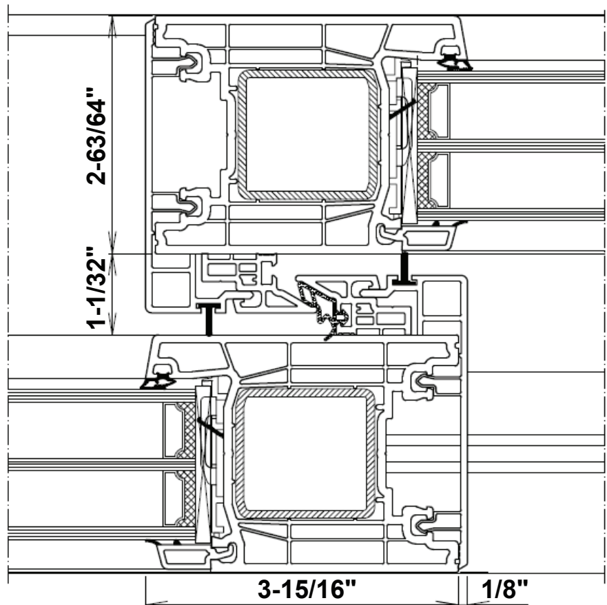
Premium HST K76 Central sash
