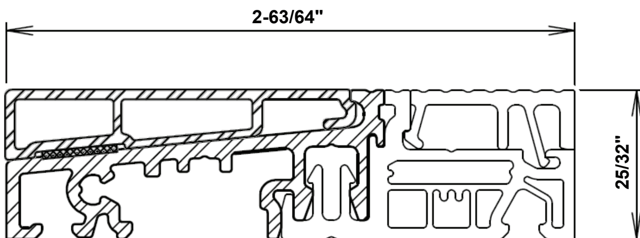
Outward opening door's sill 2-63/64"
