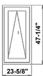
Tilt only
