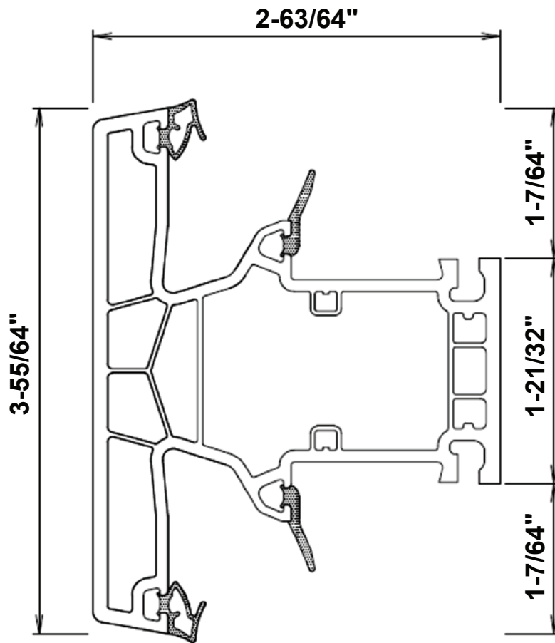
3-55/64" T-profile for frame only
