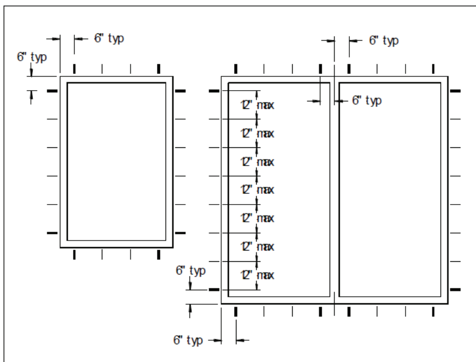
Typical anchor spacing – composite (one piece) frames - Figure 5
