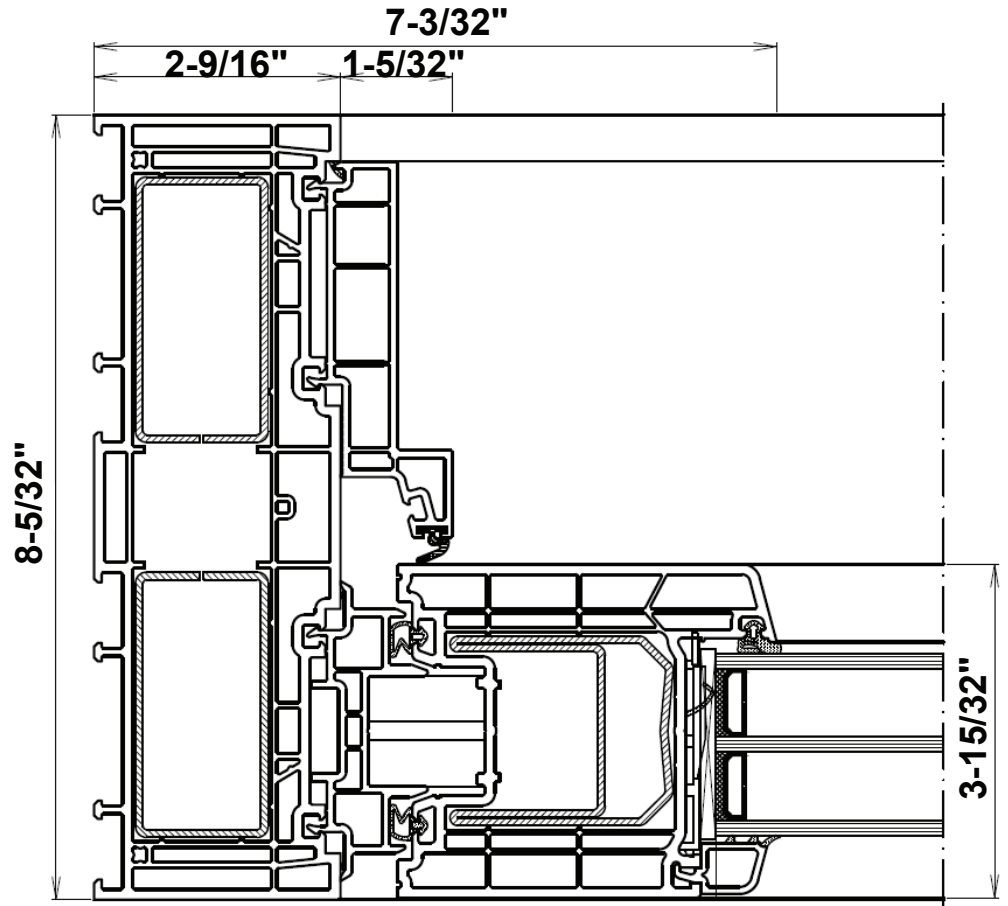
Premium HST 88 Side frame
