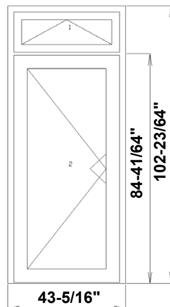
Single sash door with window in sash
