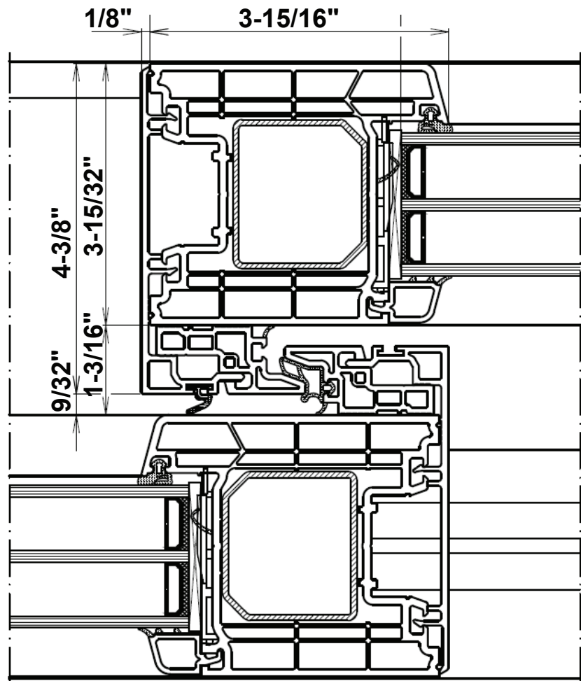
Premium HST K88 Central sash
