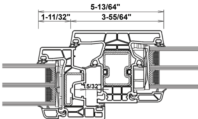
3-55/64" T-profile for frame only
