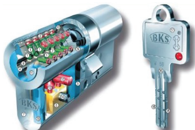
High security steel cylinder
