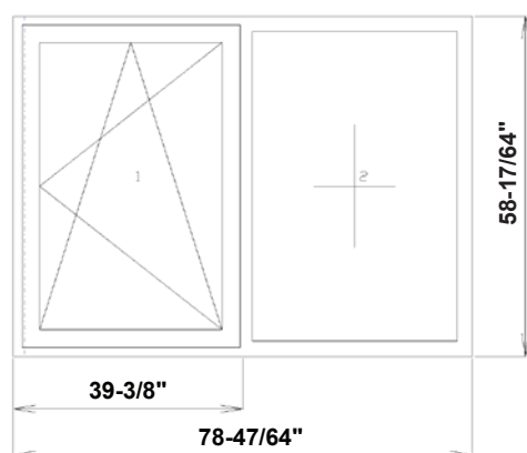
1 sash open over side fixed
