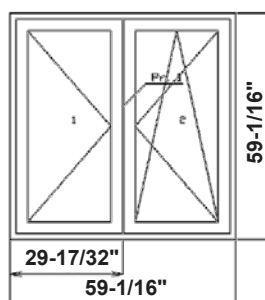
Tilt & turn 2 sash
