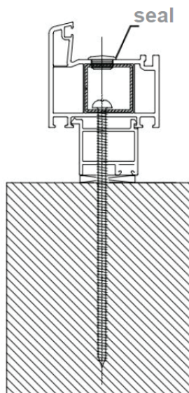
Self tapping screw
