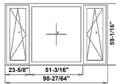
Tilt & turn sides with center fix
